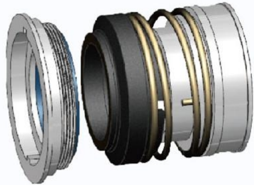
AS-92B-32mm design to suit LKH Series pumps, with a flushed seal chamber
